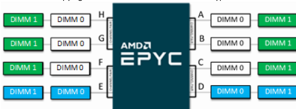
Ten DIMM Population in 2 DPC Configuration
