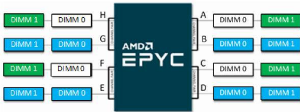
Twelve DIMM Population in 2 DPC Configuration
