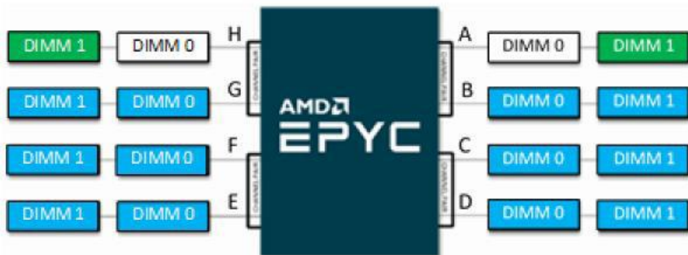
Fourteen DIMM Population in 2 DPC Configuration
