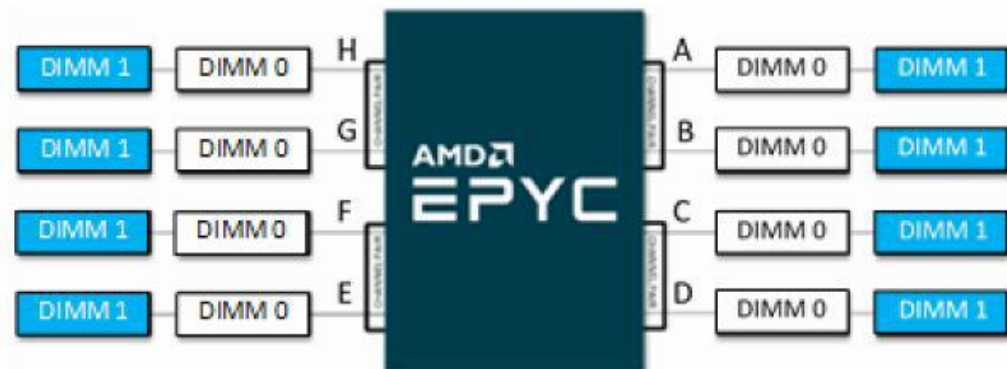
Eight DIMM Population in 2 DPC Configuration
