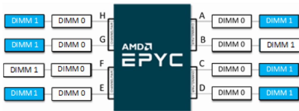
Six DIMM Population in 2 DPC Configuration
