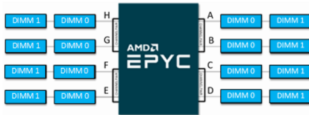
Sixteen DIMM Population in 2 DPC Configuration
