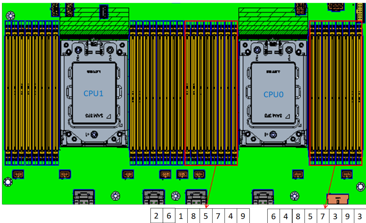
Single Socket DIMM Population Ordering in 2 DPC Configuration
