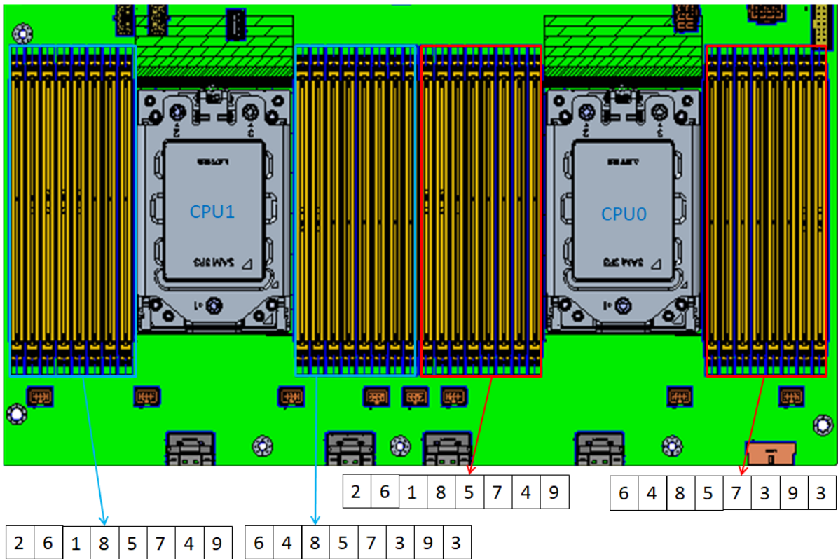
Dual Socket DIMM Population Ordering in 2 DPC Configuration
