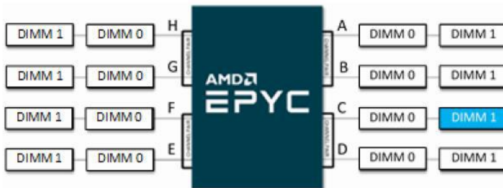
One DIMM Population in 2 DPC Configuration
