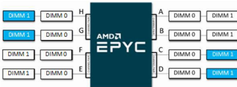
Four DIMM Population in 2 DPC Configuration
