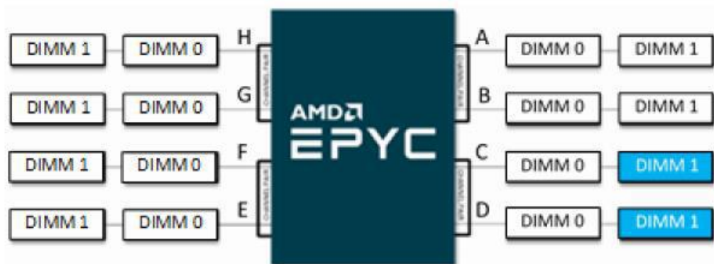
Two DIMM Population in 2 DPC Configuration
